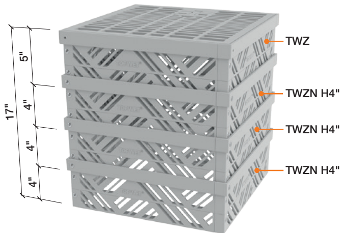
Chamber components with perforated grid, height 17"
