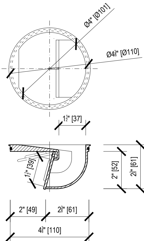
MECHANICAL STINK FLAP DN 110
